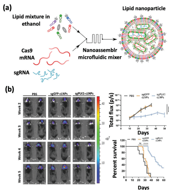
Fig. 4 (a) Schematic illustration of the synthesis of Cas9 mRNA and sgRNA-loaded lipid nanoparticles by a nanoassembly microfluidic mixer. (b) Bioluminescence images show that the nanoformulation treatment can inhibit tumor growth and enhance the mouse survival rate. This figure has been adapted/reproduced from ref. 48 with permission from the American Association for the Advancement of Science, copyright 2020.
