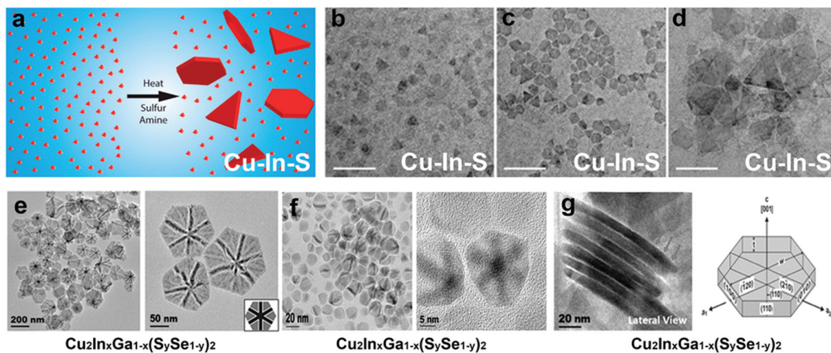
Fig. 8 (a) Schematic representation of the formation of Cu–In–S nanosheets generated via oriented attachment of CuInS 2 nanopyramids, TEM image depicting the evolution of the nanosheets collected after (b) 1 min, (c) 2 min (d) 5 min; Reproduced from ref. 21 with permission from ACS, copyright 2017; (e) TEM image of the Cu 2 In x Ga 1-x (S y Se 1-y ) 2 disc with bend contours synthesised using TOPO as the coordinating solvent, (f) TEM image of the Cu 2 In x Ga 1-x (S y Se 1-y ) 2 disc with shallow bend contours synthesised using TOPO and OLA as the solvent, (g) TEM image showing lateral view of the nanodisc where the cartoon depicts the prismatic and basal planes. Reproduced from ref. 54 with permission from ACS, copyright 2018.
