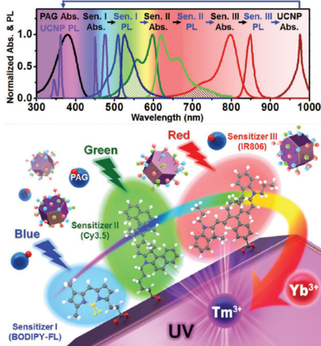
Fig. 5 Design of multi-dye-sensitized UCNPs for wide-range photo-absorption and upconversion. Reprinted with permission from ref. 107. Copyright 2016 Wiley-VCH Verlag GmbH & Co. KGaA.
