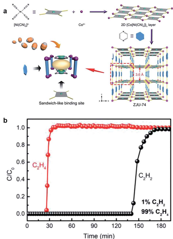
Fig. 8 (a) The construction process of ZJU-74a, 3D framework, and sandwich-like binding sites. (b) Experimental column breakthrough curves for a 1/99 \text{C}_2\text{H}_2/\text{C}_2\text{H}_4 mixture at 298 K and 1 bar. 68 Reproduced from ref. 68 with permission, copyright John Wiley and Sons, 2020.
