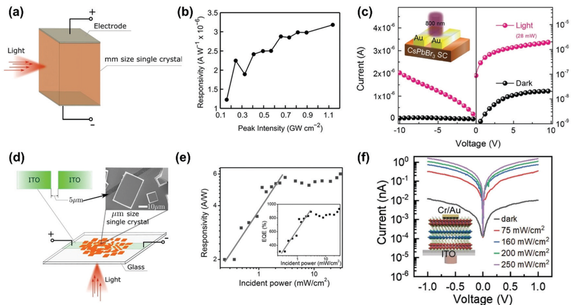
Fig. 22 (a) Photodetector schemes based on a mm-size lead halide perovskite single crystal. (b) Excitation intensity dependent responsivity of a \text{CH}_3\text{NH}_3\text{PbBr}_3 single crystal-based sub-bandgap photodetector. (c) I - V and I - V logarithm characteristics of a sub-bandgap photodetector in the dark and under 800 nm (28 mW) illumination. Inset: Schematic diagram of an IR photodetector device structure. (d) Photodetector scheme based on a \mu\text{m} -size lead halide perovskite single crystal. (e) Power-dependent responsivity ( R ) and EQE under V = 3 V bias and \lambda_{\text{ex}} = 800 nm. (f) The I - V characteristics of the 2D perovskite heterostructure device with a thickness of 20 \mu\text{m} in the dark and under 980 nm laser irradiation with different powers. Inset is schematic of the photodetector based on the n = 1/n = 2 heterostructure. (b) Reprinted with permission from ref. 59. Copyright 2015 American Chemical Society. (c) Reprinted with permission from ref. 100. Copyright 2017 Wiley-VCH Verlag GmbH & Co. KGaA, Weinheim. (e) Reprinted with permission from ref. 89. Copyright 2017 Wiley-VCH Verlag GmbH & Co. KGaA, Weinheim. (f) Reprinted with permission from ref. 70. Copyright 2019 Wiley-VCH Verlag GmbH & Co. KGaA, Weinheim.
