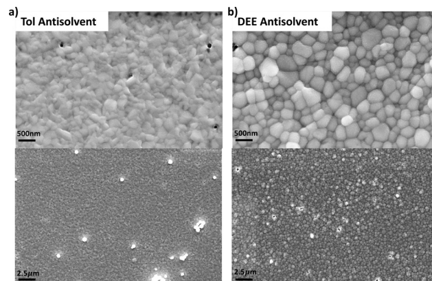
Fig. 1 The role of antisolvent on FASnI 3 morphology. Top-view SEM micrographs at 50k (top) and 10k (down) magnification of FASnI 3 thin films deposited on water-free PEDOT formulation by employing (a) toluene (Tol) and (b) DEE as antisolvent.
