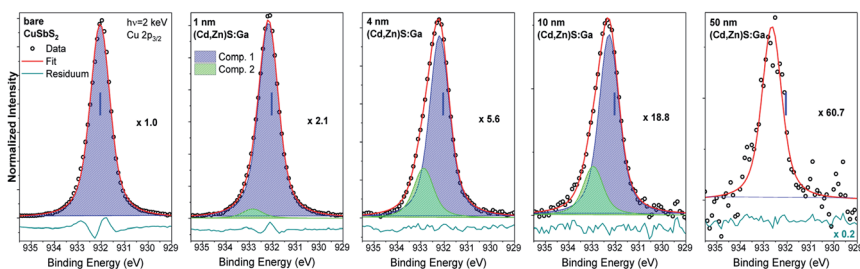
Fig. 3 Cu 2p_{3/2} HAXPES detail spectra recorded with 2 keV of the bare \text{CuSbS}_2 absorber (leftmost panel) and of the (\text{Cd,Zn})\text{S}:\text{Ga}/\text{CuSbS}_2 samples with buffer thicknesses varying from 1 nm (panel second from left) to 50 nm (rightmost panel). Spectra have been normalized to the background at low BE. The background-subtracted data is shown together with the fits and resulting residuals ( i.e. , [data – fit] – shown on different scale if required with scaling factor indicated as e.g. , \times 0.5 ). Additionally, the magnification factors are stated (as e.g. , \times 1.0 ) that were applied to show all spectra on the same intensity scale as that of the bare absorber. The vertical blue line indicates the BE position of the peak location in the spectrum of the absorber.
