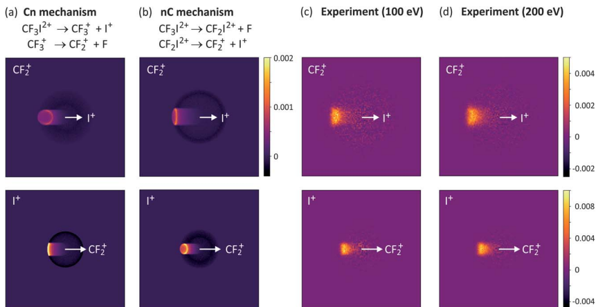
Fig. 3 Simulated covariance-map images for the unimolecular dissociation of \text{CF}_3\text{I}^{2+} for an (a) initial charge separation (mechanism 10), labelled Cn and a (b) deferred charge separation (mechanism 10), labelled nC process, compared with (c) and (d) experimentally measured covariance maps recorded at electron energies of 100 eV and 200 eV, respectively. For the top row of covariance maps, \text{I}^+ is the reference ion and \text{CF}_2^+ is the signal ion, and vice versa for the bottom row. (a)–(c) are reprinted with permission from ref. 56. Copyright 2020 Taylor & Francis Ltd.
