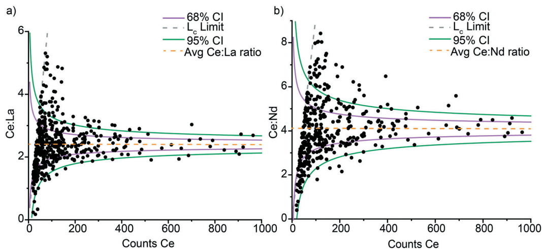
Fig. 4 Signal ratios—Ce : La (a) and Ce : Nd (b)—from Ce-NNPs are plotted against the recorded counts of Ce in each mm-NP event. These ratios follow estimated Poisson–Normal error; pink confidence interval (CI) bands for 68% CI ( \pm 1\sigma ) and the green bands for 95% CI ( \pm 1.96\sigma ) contain most of the particle events. The dashed lines represent the maximum Ce : La and Ce : Nd ratios possible as a function of counts Ce and the L_{c,sp} for La and Nd, respectively. The ratio plots converge to average ratios of 2.4 : 1 (Ce : La) and 4.1 : 1 (Ce : Nd).
