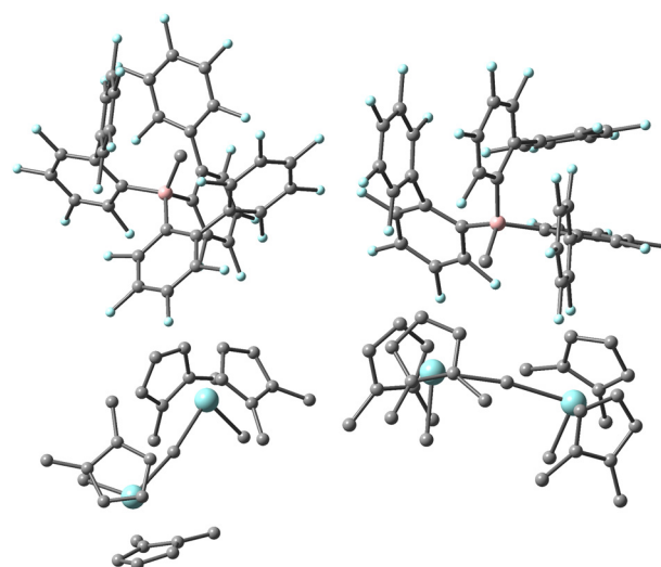
Fig. 4 X-ray structure of [(\text{Cp}''_2\text{ZrMe})_2\mu\text{-Me}][\text{MePBB}] ( \text{Cp}'' = 1,2\text{-Me}_2\text{C}_5\text{H}_3 , \text{PBB} = \text{tris}(\text{perfluorobiphenyl})\text{borane} ) (left) and thermodynamically most stable structure (right) located by DFT. Zr and F in blue, B in pink, C in grey, H omitted for clarity.
