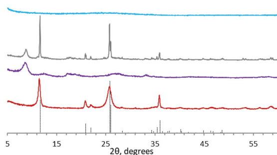
Fig. 2 Powder XRD patterns of the synthesised TiP products: aTiP – sample 4, LTP-H – sample 3, TiP1-H – sample 1 and \alpha -TiP – sample 2 (adapted from ref. 35). The dotted line represents the referenced pattern of \alpha -TiP (ref. 4).
