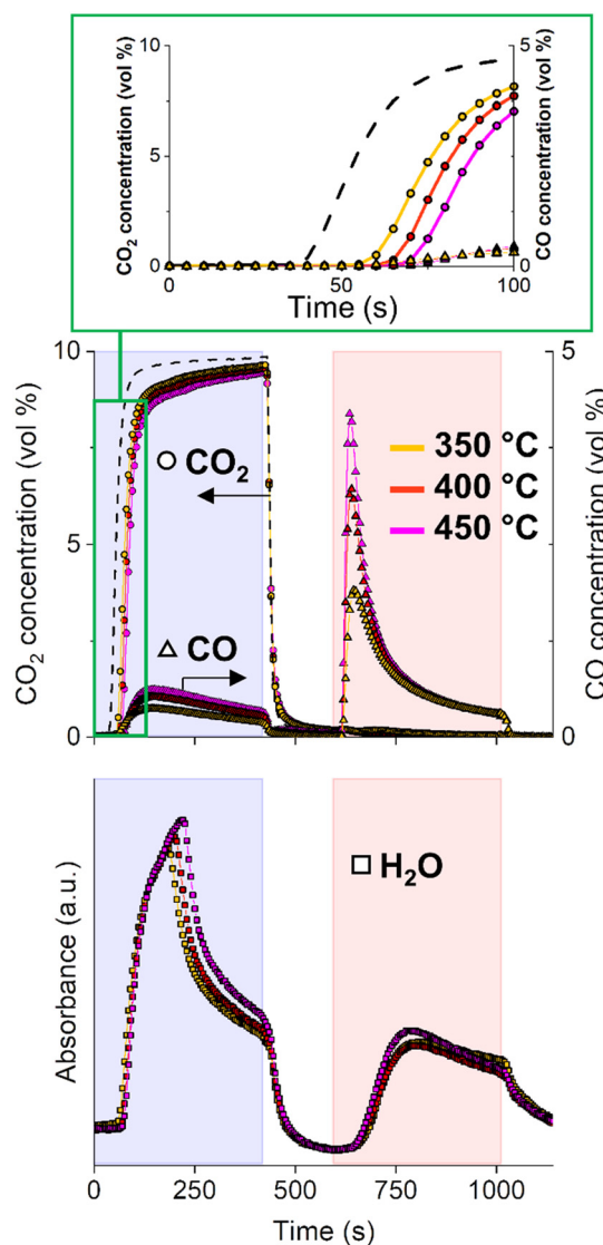
Fig. 2 Outlet gas concentrations of CO 2 (○) and CO (△) and signal of H 2 O (□) during CCR performed at 350 °C (yellow profiles), 400 °C (red profiles), 450 °C (magenta profiles). Results are averaged of 18 CCR cycles. CO 2 blank signal (dotted line) obtained as average of 2 CCR cycles during blank experiment at room temperature.
