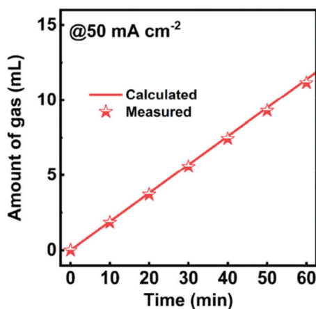
Fig. 154 Theoretically calculated and experimentally measured \text{O}_2 amounts for NCFPO/C@CC as a function of time in the NaCl + KOH electrolyte. Reproduced with permission from ref. 1858. Copyright ACS 2020.
