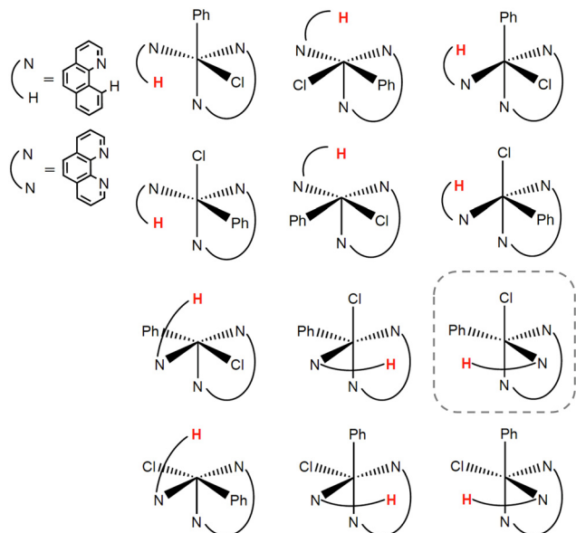
Fig. 2 Stereoisomers of the Fe(bqn)(phen)(Ph)Cl complex (bqn – \alpha -benzoquinoline, phen – 1,10-phenanthroline, Ph – phenyl). The hydrogen atom of the activated C(sp 2 )-H bond is shown in red. The lowest energy stereoisomer is in the dashed box.
