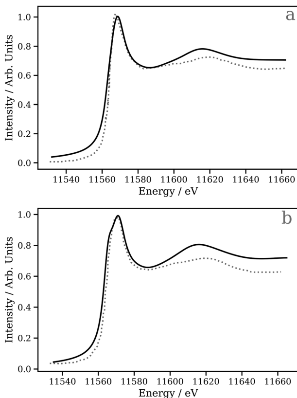
Fig. 6 The Pt L 3 edge XANES spectra of (a) [Pt(PH 3 ) 2 (η 2 -C 2 H 4 )] and (b) [Pt(PH 3 ) 2 (η 2 -C 2 (CN) 4 )]. The dashed lines are experimental Pt L 3 edge XANES spectra digitised from ref. 95 and the solid lines are DNN predictions.
