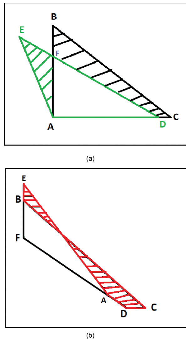
Fig. 2 The geometry of the localized electrons in a helium atom is described at large- D limit. Without inter-electronic correlation the electrons B and C are orthogonal with respect to the nucleus A. Whereas, with correlation the inter-electronic angle \angle DAE becomes slightly larger than \pi/2 . At the top panel (a), we draw the triangles formed by the two electrons and the nucleus with (\triangle CAB) and without correlation (\triangle DAE) . At the bottom (b), the area difference between the two triangles is described by the striped red region.
