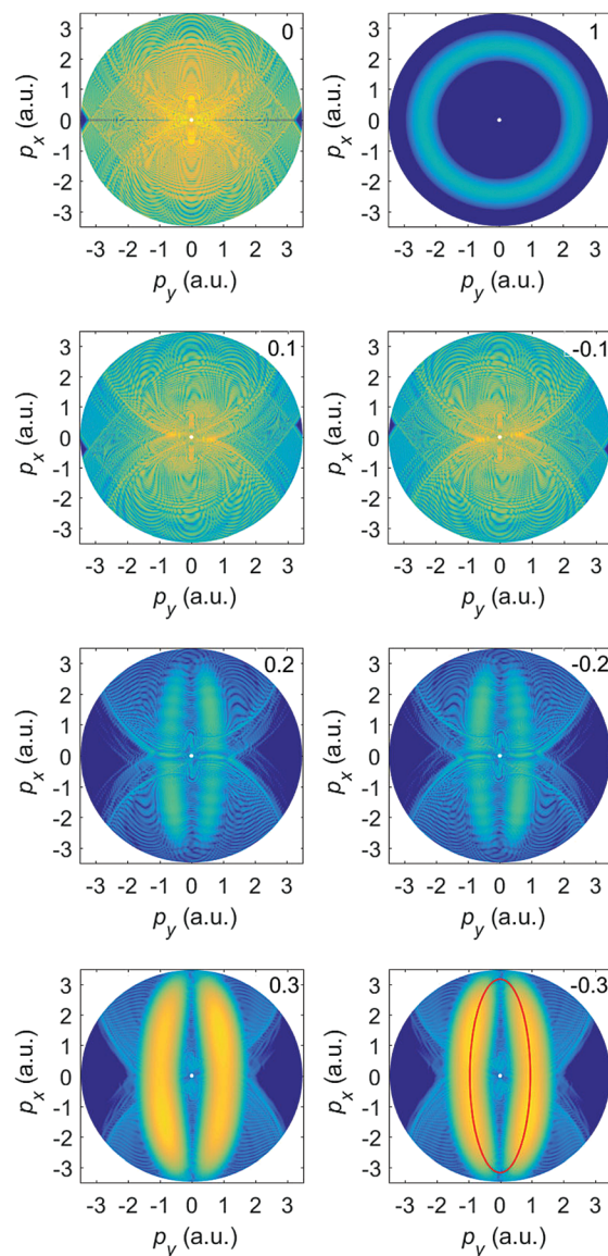
Fig. 5 The logarithm of the differential ionization rate (in a.u.) of Ar atoms for the rescattered electrons, presented in false colors in the photoelectron momentum plane, for ionization by an elliptically polarized field with wavelength 2000 nm and intensity 2 \times 10^{14} \text{ W cm}^{-2} , with the ellipticities given in the upper right corner of each panel. The false-color scale covers 6 orders of magnitude (the logarithm of the rate is between -9 and -15 ), except for the bottom panels for which it covers 8 orders of magnitude (the logarithm of the rate is between -11 and -19 ). In the bottom right panel the vector potential of the laser field is depicted by a red line.
