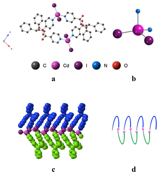
Fig. 5 For \text{L-CdI}_2 a) portion of the X-ray structure of \text{L-CdI}_2 b) environment around the \text{Cd}^{2+} cations c) the 1D helicoidal coordination polymer, projection in the xOz plane, and d) schematic representation of the helical 1D structure. H atoms and chloroform solvent molecules are not represented for clarity.
