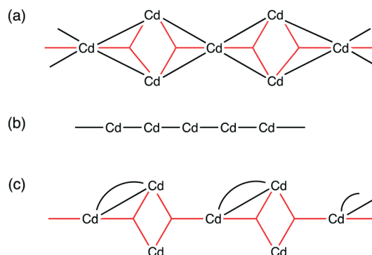
Fig. 9 Schematic representations of the chain SBUs in compounds (a) 4, (b) 5 and (c) 6. The black lines/curves represent \mu_2 carboxylates and the red three-pointed stars represent \mu_3 carboxylates.
