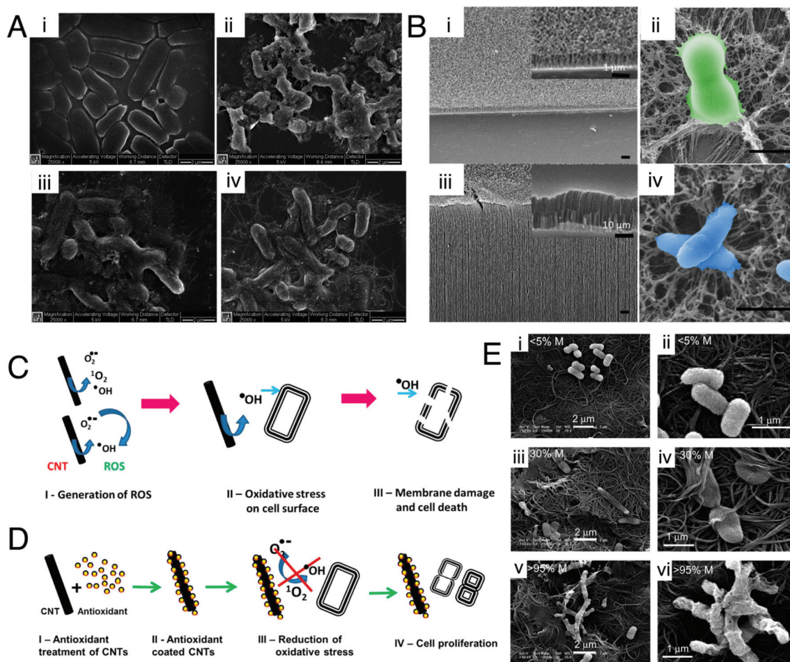
Fig. 8 Mechanism of antibacterial action of 1-D nanotubes. (A) SEM images of Salmonella cells (i) without SWCNTs, and the aggregates of cells SWCNTs of (ii) <1\ \mu\text{m} , (iii) 1\text{--}5\ \mu\text{m} , and (iv) \sim 5\ \mu\text{m} . Reproduced with permission. 221 Copyright 2007, American Chemical Society. (B) SEM images contrasting the heights of the high aspect ratio nanotubes (i) 1\ \mu\text{m} and (ii) 30\ \mu\text{m} VACNTs. False color SEM images of (iii) S. aureus and (iv) P. aeruginosa attached onto VACNT surfaces, revealing the bending of the CNTs and deformation of the bacterial cell membrane. Reproduced with permission. 222 Copyright 2018, American Chemical Society. (C) Oxidative stress (ROS)-mediated bacterial cell death. Reproduced with permission. 225 Copyright 2014, American Chemical Society. (D) Protection of bacterial cells against oxidative stress by an antioxidant. Reproduced with permission. 225 Copyright 2014, American Chemical Society. (E) Representative SEM images of E. coli deposited on SWNT filters. E. coli were deposited on the SWNT filter, incubated for 45 min in isotonic saline, and fixed with glutaraldehyde and osmium tetroxide prior to SEM imaging: (i and ii) <5\% metallic, (iii and iv) 30% metallic, and (v and vi) >95\% metallic. Note the differences in cell membrane hydration, structure, and roughness between the three samples. Reproduced with permission. 226 Copyright 2010, American Chemical Society.
