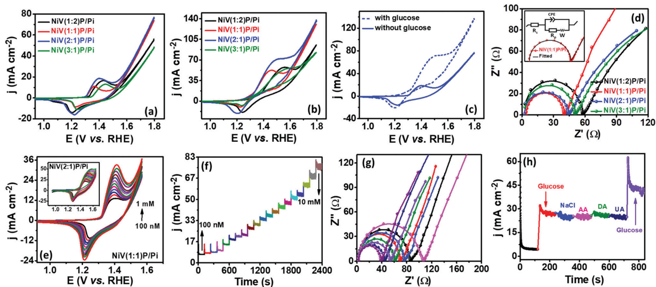
Fig. 2 CV of various NiV(P)/Pi (a) without and (b) with 10 mM of glucose, and (c) comparison of NiV(2:1)P/Pi in 0.1 M NaOH electrolyte at a scan rate of 5 \text{ mV s}^{-1} , (d) corresponding EIS studies (inset: fitted equivalent circuit of NiV(1:1)P/Pi); (e) CV (inset: CV of NiV(2:1)P/Pi), (f) chronoamperometric, and (g) EIS response of NiV(1:1)P/Pi on Ni foam in 0.1 M NaOH electrolyte at various conc. of glucose, EIS at frequency ranging from 20 mHz to 3 MHz, (h) chronoamperometric response curve of NiV(1:1)P/Pi after the successive addition of 1 mM glucose, 1 mM NaCl, 1 mM AA, 1 mM DA, 1 mM UA and 1 mM glucose in 0.1 M NaOH solution, CE: Pt wire, RE: double junction Ag/AgCl/3 M KCl.
