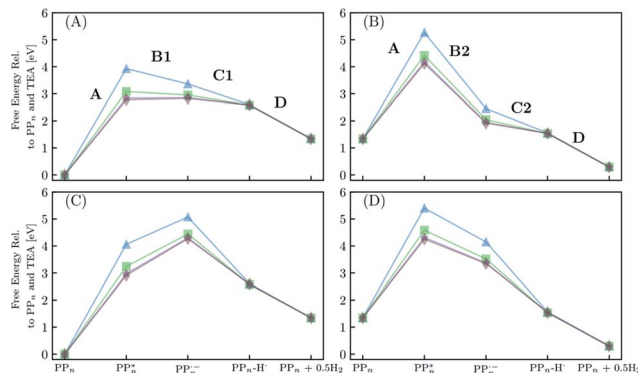
Fig. 8 The predicted free energy profile for each step in H_2O of sub-cycle I (A) and II (B). The predicted free energy profile for each step in TEA of sub-cycle I (C) and II (D). Data shown for n = 2 (blue triangles), 4 (green squares), 6 (purple stars) and 7 (brown diamonds), calculated using B3LYP and provided relative to PP_n and TEA. The x-axis labels omit any reference to the SED or its degradation products. For the equivalent data calculated with CAM-B3LYP see Fig. S3†
