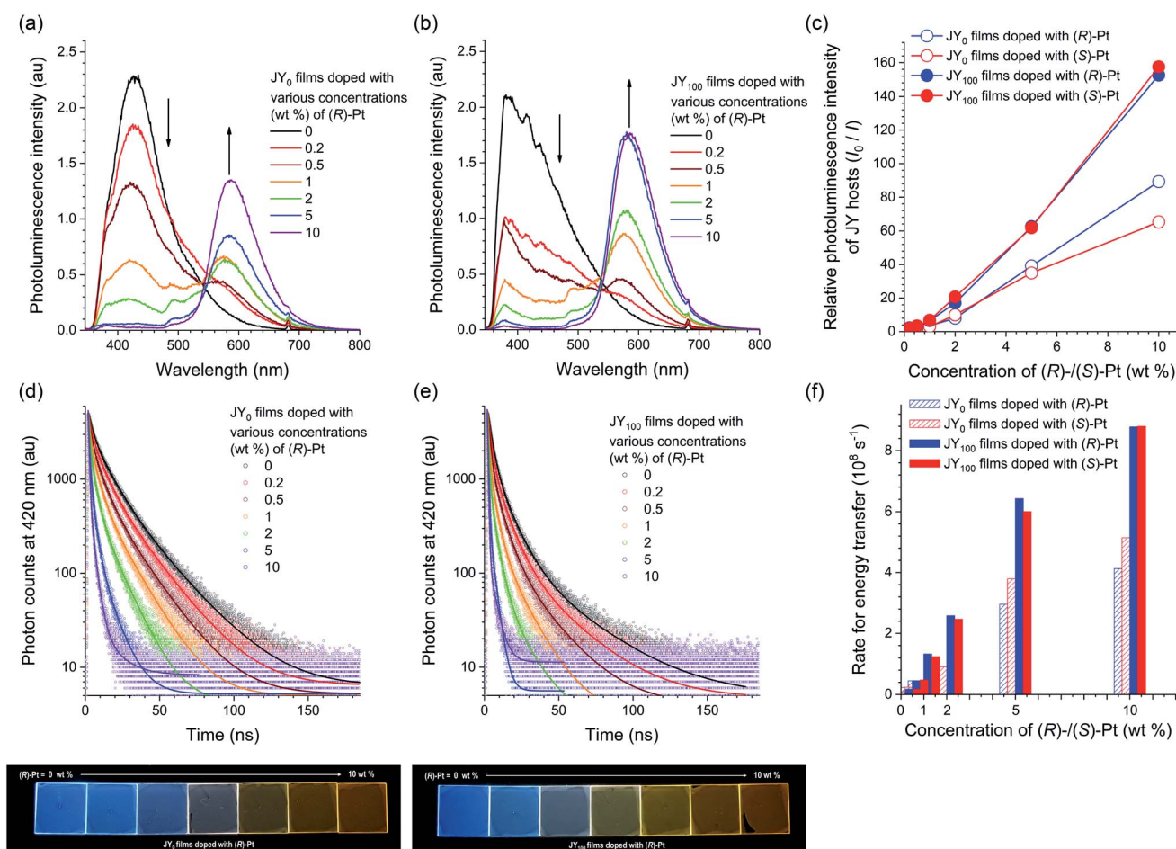
Fig. 6 (a and b) Photoluminescence spectra ( \lambda_{ex} = 339 nm) for JY 0 (a) and JY 100 (b) films doped with various concentrations (0–10 wt%) of (R)-Pt. The spectra of the films doped with (S)-Pt are shown in ESI, Fig. S9.† (c) Ratios of the photoluminescence intensities of the JY n hosts in the absence of the presence of increased concentrations of the Pt dopants ( I_0/I ). (d and e) Photoluminescence decay traces ( \lambda_{obs} = 420 nm) of JY 0 (d) and JY 100 (e) films doped with various concentrations (0–10 wt%) of (R)-Pt obtained after picosecond pulsed laser photoexcitation at 377 nm (temporal resolution = 25 ps). The solid curves are nonlinear least-squares fits to a biexponential decay model. The decay traces of the films doped with (S)-Pt are shown in ESI, Fig. S9.† The decay traces of dopant emissions recorded at a wavelength of 590 nm are shown in ESI, Fig. S10.† The bottom photographs show the photoluminescence emissions of JY 0 (left) and JY 100 (right) films doped with various concentrations of (R)-Pt visualized under photoirradiation at a wavelength of 365 nm. (f) Rates of energy transfer ( k_{ET} ) from the JY hosts to the Pt dopants.
