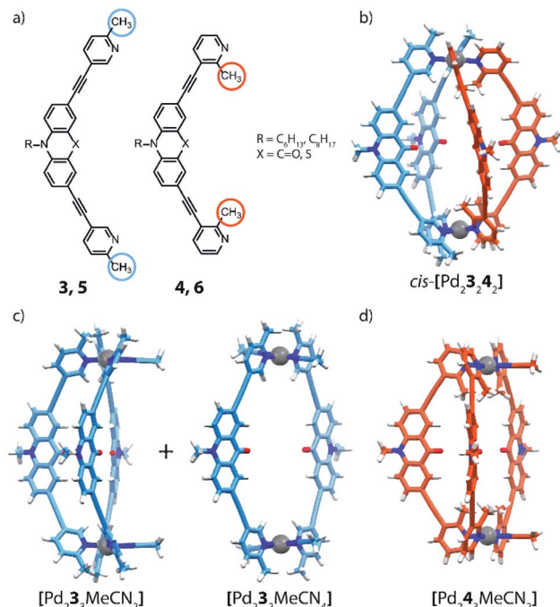
Fig. 5 (a) Banana-shaped ligands with outside- and inside-pointing methyl groups; (b) DFT model of heteroleptic cage cis -[Pd 2 L 3 4 2 ]; (c) DFT model of bowl and ring obtained with ligand 3 and (d) bowl obtained with ligand 4 .
