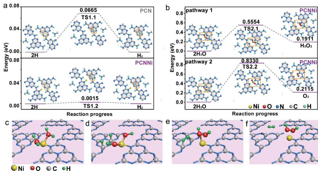
Fig. 6 Reaction pathways of (a) water reduction to H_2 and (b) water oxidation to H_2O_2 (top) and O_2 (down) for PCNNi (single-atom Ni coordinated with sp^2 NA atoms). (c–f) Proposed mechanisms of photocatalytic pure water splitting into H_2 and H_2O_2 for PCNNi (single-atom Ni coordinated with sp^2 NA atoms).
