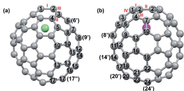
Fig. 7 Different types of carbon atoms in (a) Th@C 3v (8)-C 82 and (b) U@C 2v (9)-C 82 .
