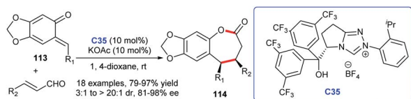
Scheme 35 The synthesis of benzo- \epsilon -lactones.
