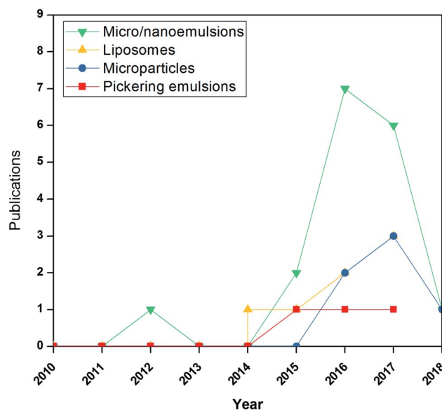
Fig. 5 Number of publications indexed by scopus (www.scopus.com) based on search strings related to the use of "emulsions", "nano-emulsions", "liposomes", "microparticles", "Pickering emulsions" and "active films" in the title, keywords, and abstract of the publication.
