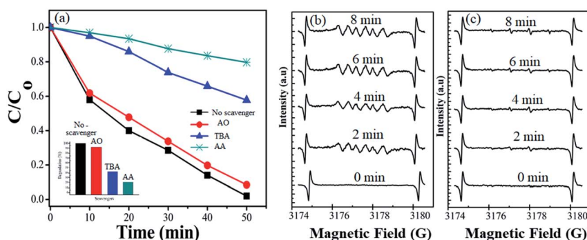
Fig. 8 (a) Effects of different radical scavengers on CV degradation over 1T-MoS 2 @(Bi 0.40 Fe 0.60 )VO 4 under visible light irradiation. (b) DMPO spin trapping EPR spectra for DMPO-•O 2 - and (c) DMPO-•OH - under visible light over 1T-MoS 2 @(Bi 0.40 Fe 0.60 )VO 4 photocatalyst.
