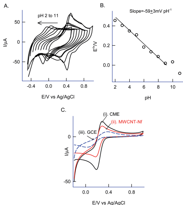
Fig. 3 (A) Effect of solution pH on the CV response of GCE/Nf-MWCNT@PhOCH 3 -Redox at a fixed v = 50 \text{ mV s}^{-1} . (B) Plot of E^\circ vs. solution pH. (C) CV responses of 5 mM Fe(CN) 6 dissolved in 0.1 M KCl on GCE/Nf-MWCNT@PhOCH 3 -Redox (i), GCE/Nf-MWCNT (ii) and GCE (iii).
