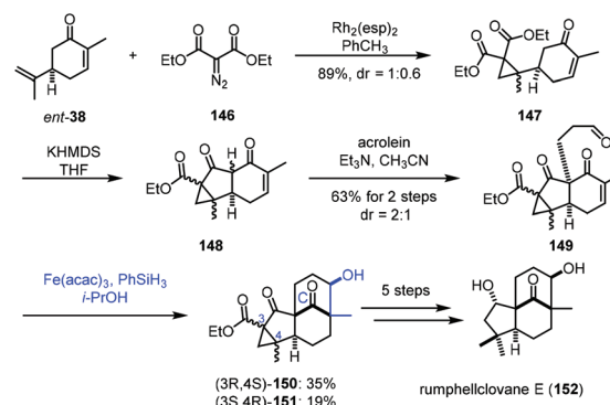
Scheme 18 Liu's synthesis of rumpHELLCLOVANE E ( 152 ).
