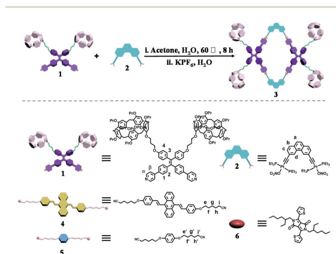
Scheme 1 Self-assembly of 120° dipyriddy donor 1 and 60° diplatinum(II) acceptor 2 into discrete rhomboidal metallacycle 3 , and the chemical structures of building block DSA-containing guest 4 , model guest 5 and fluorescent acceptor 6 .
