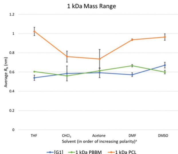
Fig. 5 Calculated average R_h values, from DOSY- ^1\text{H} NMR, for Tetra[G1] Bnz 4 , 1 kDa PCL, and 1 kDa PBBM in all tested solvents. a Solvent polarity values from Reichardt were used to determine order of polarity. 39
