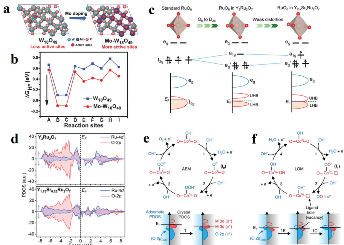
Fig. 10 (a) Different oxygen sites on W_{18}O_{49} (010) and Mo- W_{18}O_{49} (010). (b) The calculated Gibbs free energy of HER on different oxygen sites of W_{18}O_{49} and Mo- W_{18}O_{49} (010). 113 (c) Schematic illustrations of different RuO_6 along with the splitting of Ru 4d orbitals. (d) Schematic evolution of band alignments through Sr^{2+} substitution for Y^{3+} in Y_2Ru_2O_7 . 127 (e and f) Relationship between oxygen vacancy concentration and Co–O bond. 115
