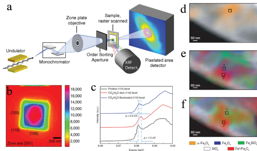
Fig. 7 (a) STXM and SAXFM setup; Copyright 2014, National Academy of Sciences; (b) SFXM image of a \text{Cu}_2\text{O} nanoparticle; Copyright 2019, Springer Nature; (c) scanning X-ray nanospectroscopy of the (110) facet; Copyright 2019, Springer Nature; (d) to (f) chemical contour images of the catalyst under different treatments; Copyright 2008, Springer Nature. All panels reproduced with permission. 148,156,160
