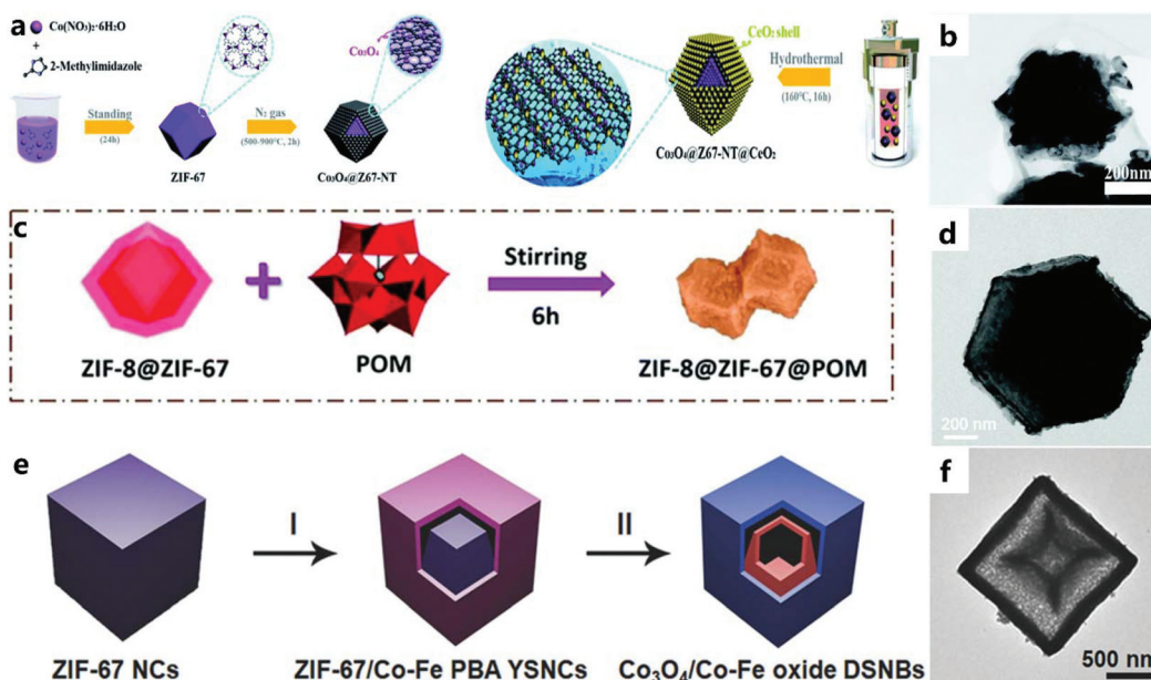
Fig. 4 (a) Synthesis route for the \text{Co}_3\text{O}_4@\text{Z67-NT}@ \text{CeO}_2 composites. (b) TEM images of \text{Co}_3\text{O}_4@\text{Z67-NT}@ \text{CeO}_2 . 68 Copyright © 2019, Royal Society of Chemistry. (c) Schematic diagram for the synthesis of \text{ZIF-8}@ \text{ZIF-67}@ \text{POM} . (d) TEM image of \text{ZIF-8}@ \text{ZIF-67}@ \text{POM} . 69 Copyright © 2019, Royal Society of Chemistry. (e) Schematic illustration of the formation process of \text{Co}_3\text{O}_4/\text{Co-Fe} oxide DSNBs. (f) TEM images of \text{Co}_3\text{O}_4/\text{Co-Fe} oxide DSNBs. 70 Copyright © 2018 Wiley-VCH Verlag GmbH & Co. KGaA, Weinheim.
