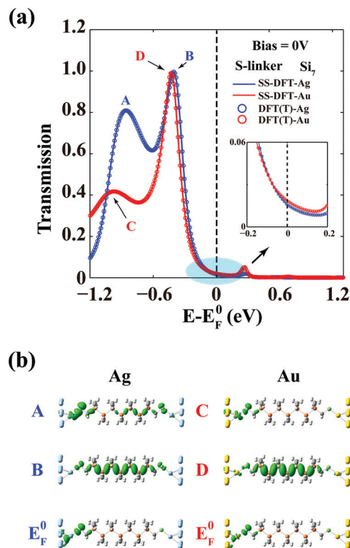
Fig. 4 Zero-bias transmission spectra of \text{Si}_7 -S-M. (a) Transmission spectra of \text{Si}_7 -S-M ( M = \text{Au}, \text{Ag} ) from SS-DFT and TransSIESTA (DFT(T)). For both the Au and Ag cases, the results from the two packages are essentially the same. Inset: enlarged view of the transmission spectra near the Fermi energy. Note that the Au contact is more conducting than the Ag contact. (b) Tunneling eigenchannels of major peaks in the transmission spectra, A and B for the Ag contact, and C and D for the Au contact. Tunneling eigenchannels at the Fermi energy were also plotted.
