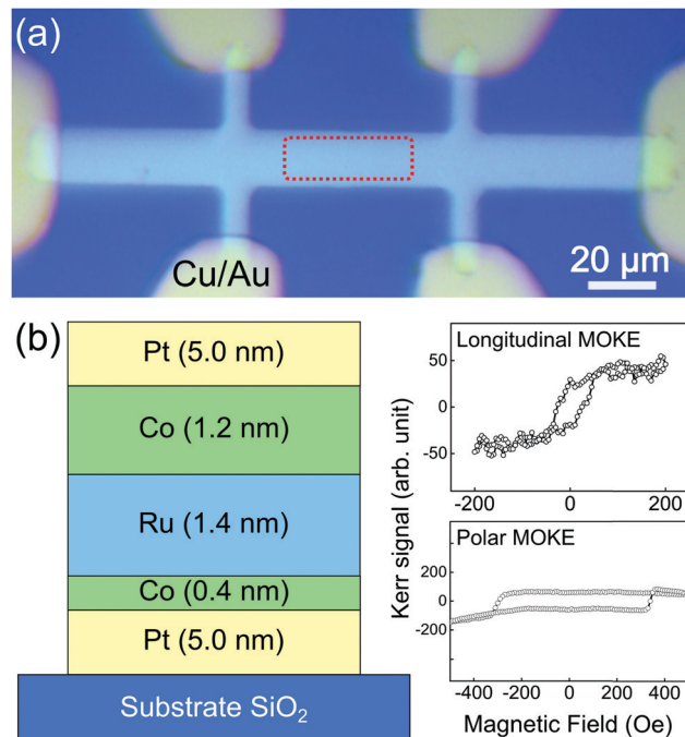
Fig. 2 (a) The optical image of the geometry of the sample. The Hall bar's length is about 200 \mu\text{m} and the width is about 20 \mu\text{m} . Electrodes were deposited composed of an alloy of Cu and Au. The red-dotted square labels the area that is illuminated by the twisted light. (b) The sandwiched structure is shown in the left part of (b).
