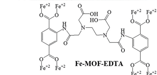
Fig. 11 Schematic representation of the fabrication of Fe-MOF-EDTA [reprinted with permission from ref. 129, Copyright © Elsevier, 2019].
