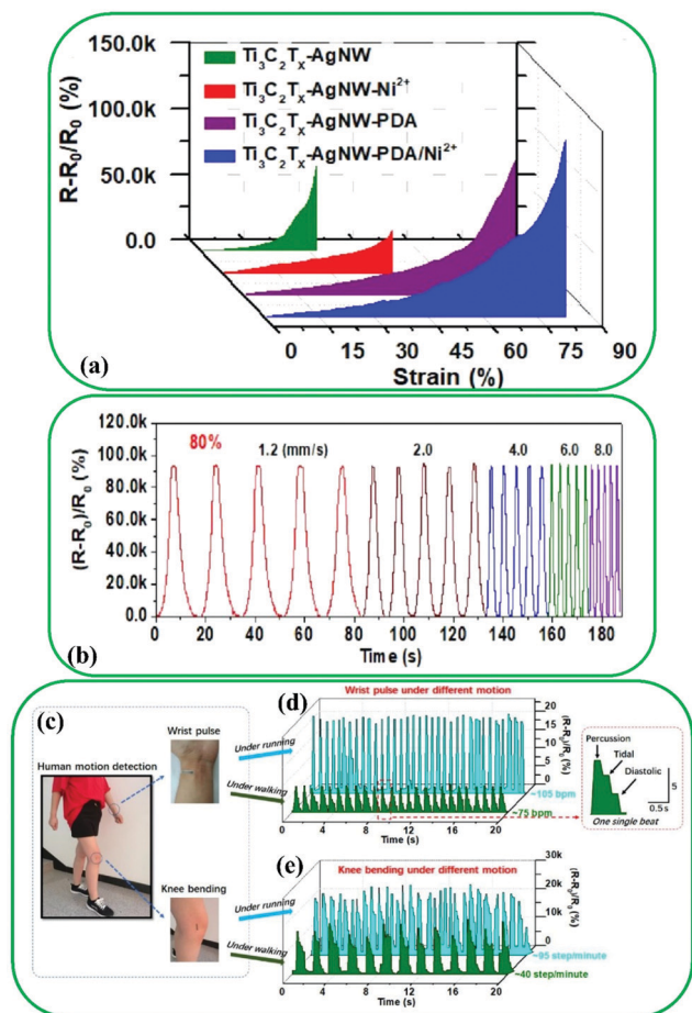
Fig. 15 (a) Typical relative resistance change vs. applied strain for the \text{Ti}_3\text{C}_2\text{-AgNW} , \text{Ti}_3\text{C}_2\text{-AgNW-PDA} , \text{Ti}_3\text{C}_2\text{-AgNW-Ni}^{2+} , \text{Ti}_3\text{C}_2\text{-AgNW-PDA/Ni}^{2+} strain sensors. (b) Relative resistance variation of the \text{Ti}_3\text{C}_2\text{-AgNW-PDA/Ni}^{2+} strain sensor under incremental strain rates cycling from 0 to 80%. Monitoring human body (knee bending and wrist pulse) under running and walking conditions by means of \text{Ti}_3\text{C}_2\text{-AgNW-PDA/Ni}^{2+} strain sensors. (c) Images of wearable strain sensors attached to the wrist and knee. (d) Relative resistance variation of a wrist pulse. (e) Relative resistance change of knee bending. Reproduced with permission. 192 Copyright 2018, American Chemical Society.
