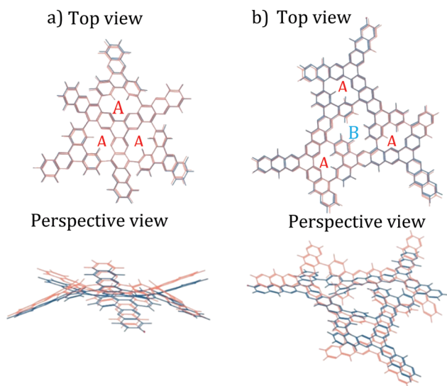
Fig. 3 Overlay between DFT-optimized B3LYP/6-31+g* (blue) and MM-optimized (UFF, orange) subsections of hypothesized DPCOF structure. (a) Subsection centered around monomer 4 . (b) Subsection centered around B pore. Perspective view illustrates the inherent curvature of DPCOF chemical “building blocks”.
