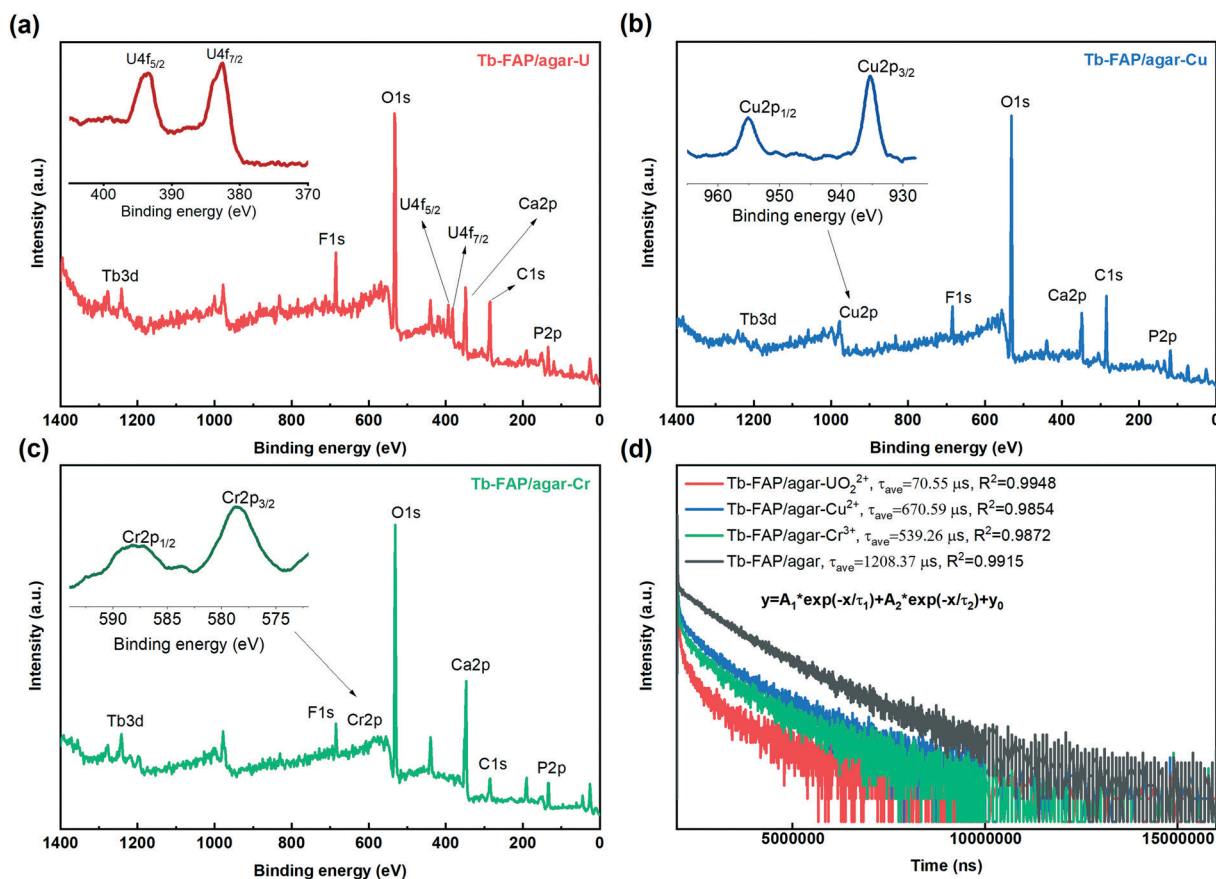
Fig. 4 XPS spectra of the Tb-FAP/agar after treatment with (a) \text{UO}_2^{2+} , (b) \text{Cu}^{2+} , and (c) \text{Cr}^{3+} accompanied with the insets showing the detailed XPS spectra of U 4f, Cu 2p, and Cr 2p, respectively. (d) The luminescence lifetime spectra of the Tb-FAP/agar sample recorded in the presence and absence of \text{Cu}^{2+} , \text{Cr}^{3+} , and \text{UO}_2^{2+} ions ( \lambda_{\text{ex}} = 377 \text{ nm} and \lambda_{\text{em}} = 543 \text{ nm} ).
