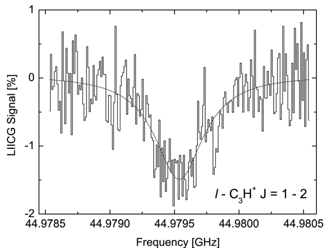
Fig. 14 The rotational transition J = 2 \leftarrow 1 of I-C 3 H + measured by storing several ten thousand C 3 H + ions in a cold (4.1 K) and dense ( \sim 10^{15} cm -3 ) helium bath and continuous irradiation with tunable narrow-band mm-wavelength radiation. The rotational transition of the bare ion can be recorded by counting the C 3 H + –He complex ions as a function of excitation frequency. On resonance, the number of formed complex ions (black histogram) decreases by about 1.5%. The black line is a fit with a Lorentzian line-shape function to the data. In the original publication, 133 the lines for J = 3 \leftarrow 2 and J = 4 \leftarrow 3 are shown.
