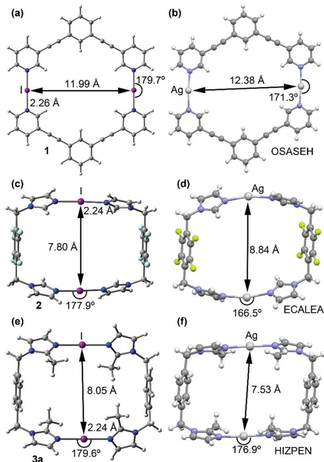
Fig. 2 Optimized geometries of compounds 1 (a), 2 (b) and 3a (c) at the M06-2X/def2TZVp level of theory. The X-ray structures of the corresponding Ag(I) metallacycles (CSD refcodes OSASEH (b) and HIZPEN (f)).
