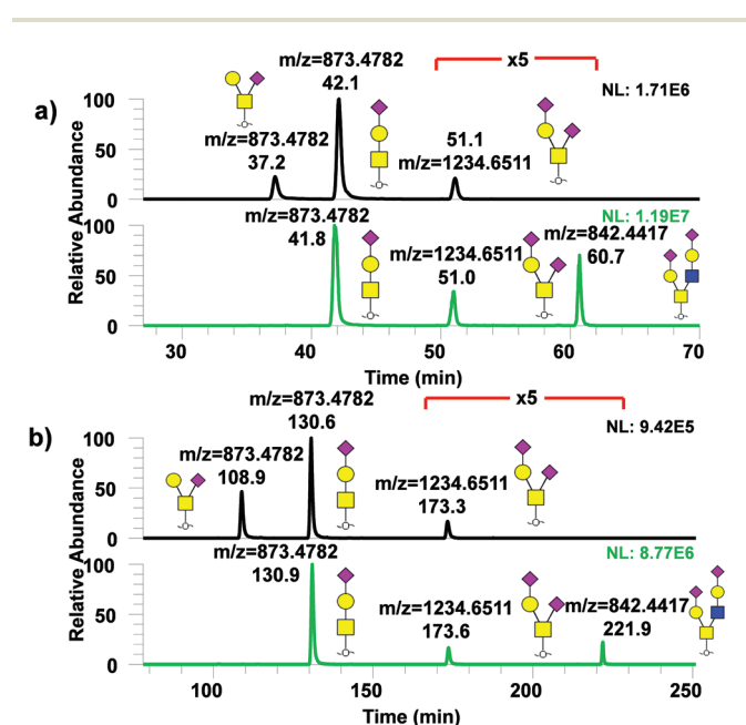
Fig. 6 Analysis of permethylated O -glycans using 50 and 200 cm \mu PAC. EIC of permethylated O -glycans derived from \kappa -casein and bovine fetuin using (a) \mu PAC 50 cm and (b) \mu PAC 200 cm. Upper panel of each figure depicts permethylated O -glycans derived from \kappa -casein and bottom panel shows permethylated O -glycans derived from bovine fetuin.
