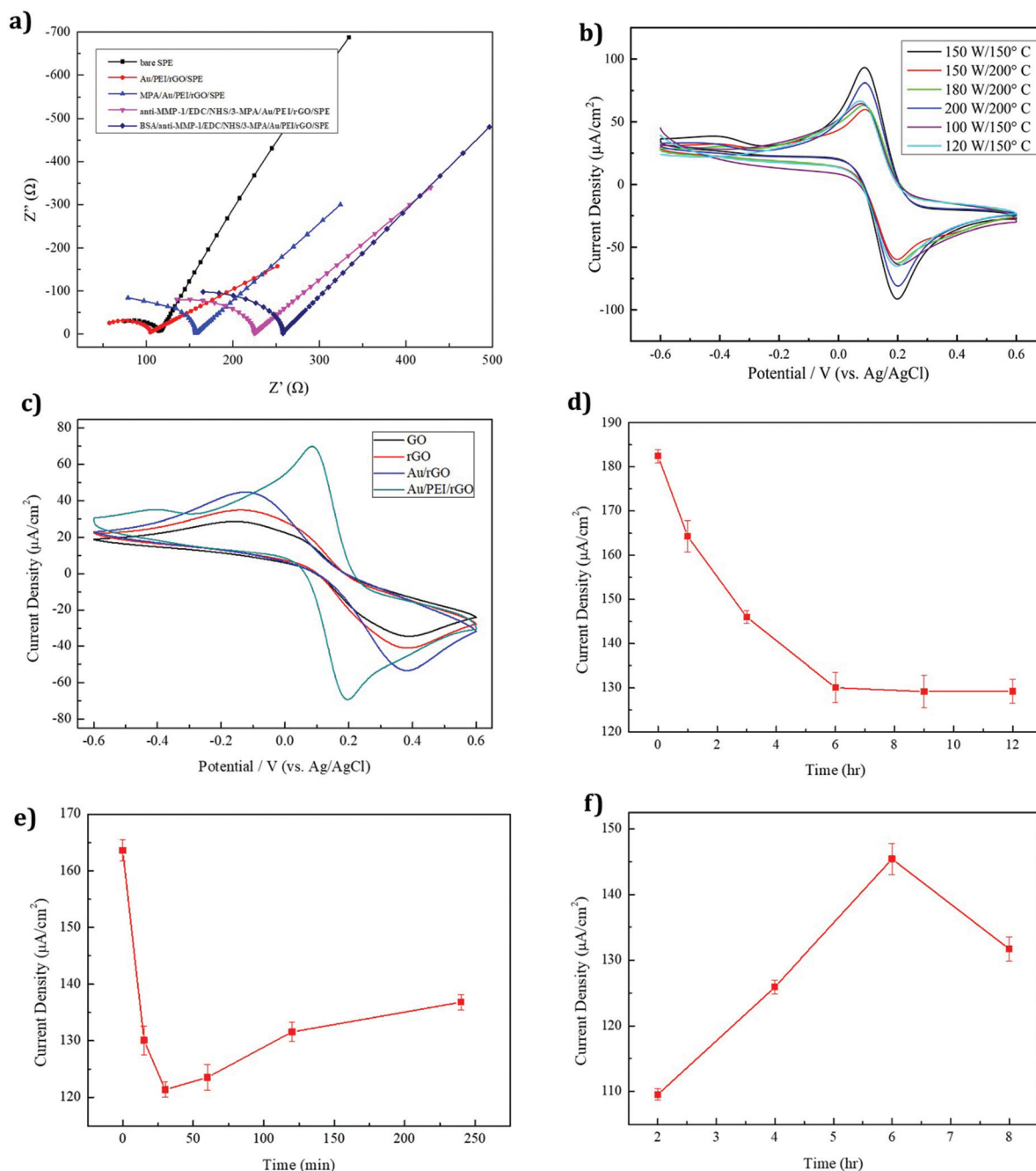
Fig. 5 (a) EIS spectra of different modified electrodes (conditions: 5 mM \text{Fe}(\text{CN})_6^{3-/4-} dissolved in 0.1 M PBS/0.1 M KCl (pH 7.4), scan rate 50 mV \text{s}^{-1} ). (b) CVs of the AuNP/PEI/rGO-modified SPE (conditions: 5 mM \text{Fe}(\text{CN})_6^{3-/4-} dissolved in 0.1 M PBS/0.1 M KCl (pH 7.4), scan rate 50 mV \text{s}^{-1} , n = 3 ) prepared under different microwave synthesis conditions. (c) CV responses of four different modified electrodes, namely GO, rGO, AuNP/rGO and AuNP/PEI/rGO-modified SPE. (d) Plot of the 3-MPA modification time versus current change. (e) Plot of the EDC/sulfo-NHS modification time (0, 15, 30, 60, 120, and 240 min) versus current change. (f) Plot of the MMP-1 antibody modification time versus current change.
