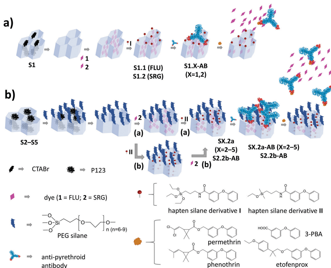
Scheme 1 Architecture and synthesis routes of the antibody-gated mesoporous materials (a) containing MCM-41 (S1) as mesoporous scaffold and (b) S2–S5 containing different types of SBA scaffolds (S2: SBA-15, conventional long fibres; S3: SBA-15 platelets; S4: SBA-15 long fibres with enlarged pores; S5: SBA-16 nanoparticles).
