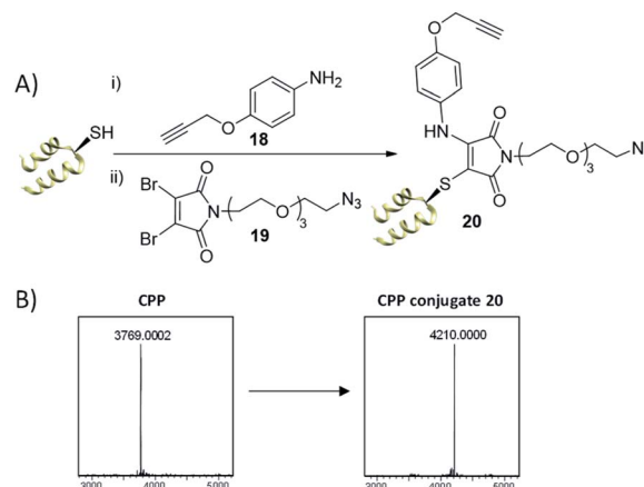
Fig. 5 (A) Dual thiol-amine conjugation on CPP. CPP (0.9 mM) in PB (10 mM, pH 6.5), amine-alkyne 18 (40 equiv.), DBM 19 (1.2 equiv.) left at 37 °C for 30 min, (B) LCMS data; expected mass for conjugate 20: 4208 Da, observed mass: 4210 Da. See ESI Fig. S19–S22† for more detail.
