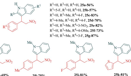
Scheme 7 Friedel-Crafts alkylation of indoles with nitroalkenes in water.
