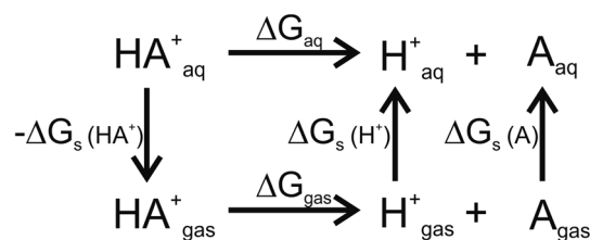
Fig. 1 Thermodynamic cycle used for \text{p}K_a calculations. \Delta G_{\text{gas}} free energy of deprotonation in gas-phase; \Delta G_s solvation free energy; \Delta G_{\text{aq}} free energy of deprotonation in aqueous solution.
